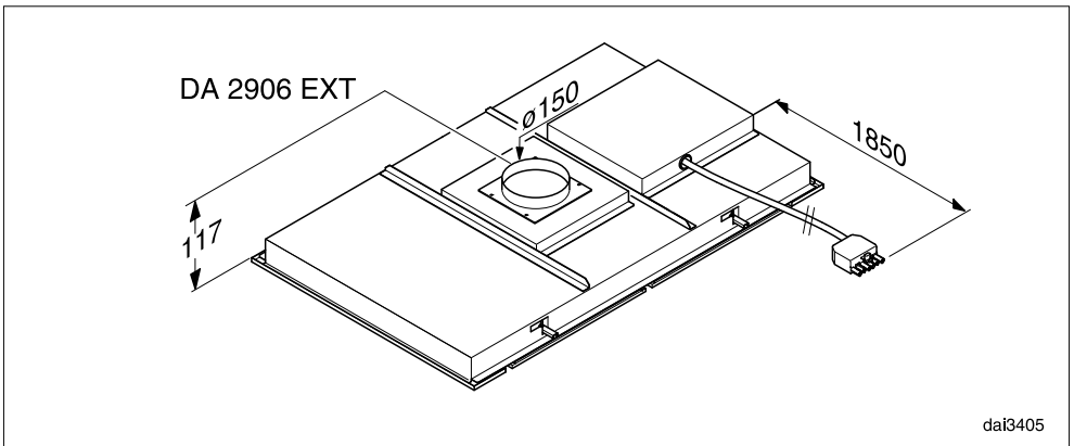
DA 2906 EXT - different appliance dimensions
