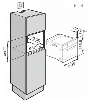
M 6262 TC, Isometry tall unit solo (installation drawings) (*footnote)
