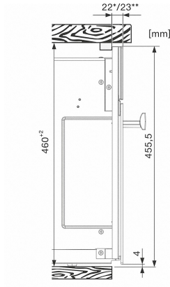
M 6262 TC, side view built-under (installation drawings) (*footnote)
