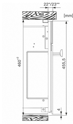
M 6262 TC, side view built-under (installation drawings) (*footnote)
