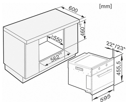
M 6262 TC, Isometry built-under (installation drawings) (*footnote)
