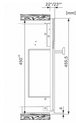
M 6262 TC, side view solo (installation drawings) (*footnote)
