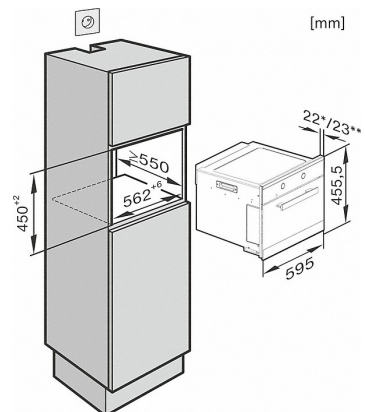
M 6262 TC, Isometry tall unit solo (installation drawings) (*footnote)
