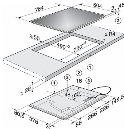
KM 6629 (Installation drawing)
