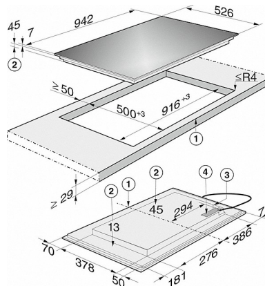
KM 6388 (installation drawing)
