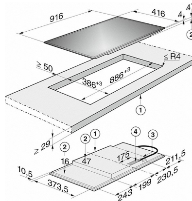
KM6381 (installation drawing)
