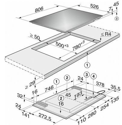
KM 6363-1 PowerFlex (Installation drawing) - LightPrint
