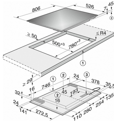
KM 6363 PowerFlex (Installation drawing) - LightPrint
