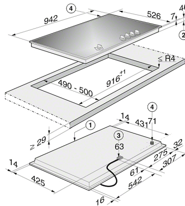
KM 3054 G (installation drawing) VG AUS
