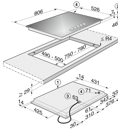
KM 3034 G (Installation drawing) VG AUS
