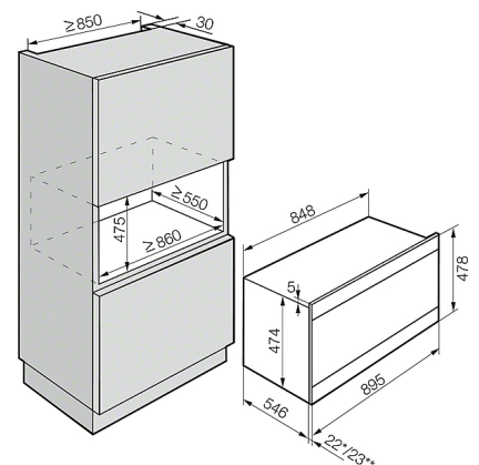
H 5981 BP, H 6890 BP - 90 cm (Installation drawing)
