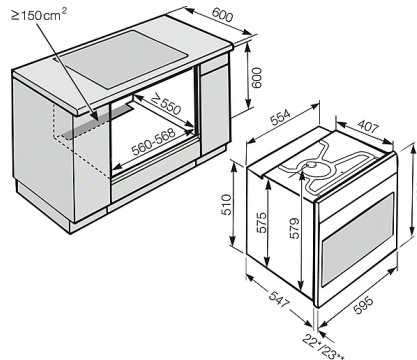
H 5000 EP/BP - 60 cm (Installation drawing)
