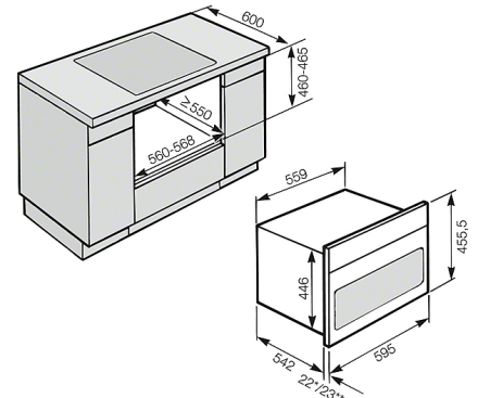
H 5000 BM, H 6000 BM - 45 cm (Installation drawing)
