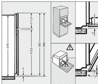
Detailed installation drawing H 6000 BPX, ArtLine, 76 Litres, (Installation drawing)
