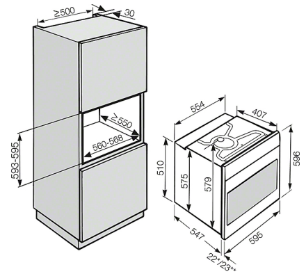
H 5000 BP; H 6000 BP; H 2000 BP; 60 cm (Installation drawing)
