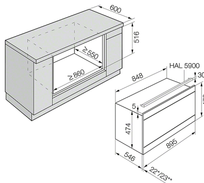
H 5900 B, H 5961 B, H 6090 B - 90 cm (Installation drawing)
