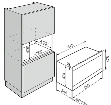
H 5900 B, H 5961 B, H 6090 B - 90 cm (Installation drawing)
