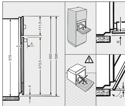
Detailed drawing H 6000, H 5000, H 4000, E/B, EP/BP, 76 litres, (Installation drawing) VG AUS, VG GB
