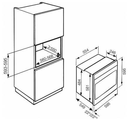
H 2000 B, H 4000 B, H 5000 B - 56 litres- 60 cm (Installation drawing)
