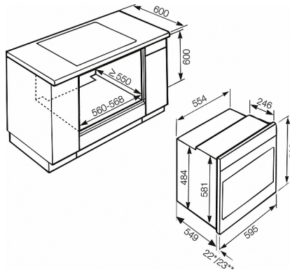
H 4000 E/B, H 2000 E/B - 50 litres- 60 cm (Installation drawing)
