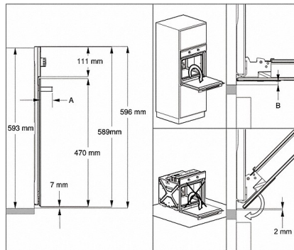
H 4000 E/B, H 2000 E/B - 50 litres- 60 cm (Installation drawing)
