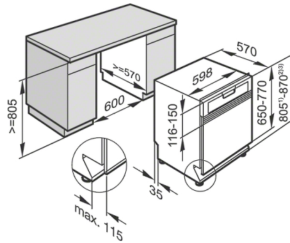
G1000/G1002/G5000/G6000 integrated dishwasher (installation drawing)
