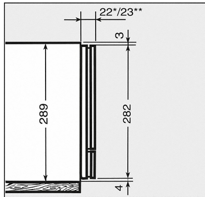
ESW 6129 X, ESW 6229 X (Installation drawing) - handleless
