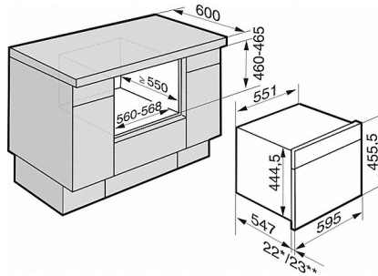
DGM 6000 (Installation drawing)
