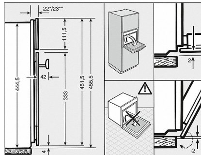
DGM 6000 PureLine (Installation drawing)
