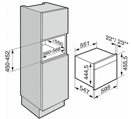
DGM 6000 (Installation drawing)
