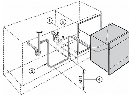
DGC 6000 built in base unit, CLST (Installation drawing)
