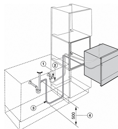
DGC 6000 built in wall unit, CLST (Installation drawing)
