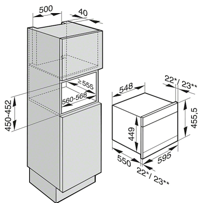
DGC 6500, DGC 6600, DGC 6800, in a tall unit, CLST (Installation drawing)
