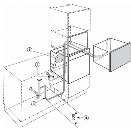
DGC 6805, plumbed connection (installation drawing)
