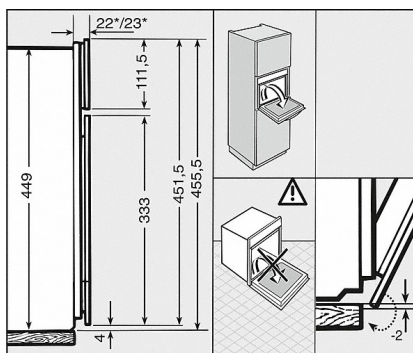
DGC 6500, DGC 6600, DGC 6800, DGC 6805 detailed installations drawing (Installation drawing) - without handles
