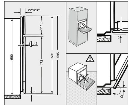
DGC 6000 XXL PureLine (detailed installation drawing)
