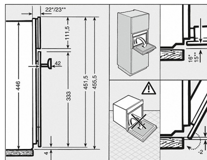
DG 6000 - detail drawing PureLine (Installation drawing)
