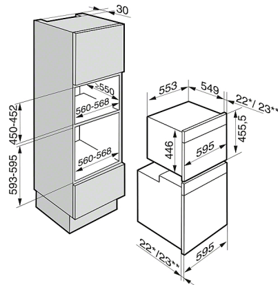
DG 6000 in combination with H 6000 (Installation drawing)
