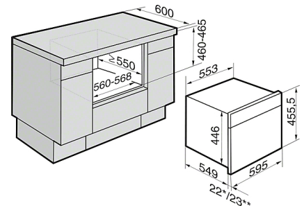
DG 6000 (Installation drawing)
