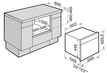
DG 6000 (Installation drawing)
