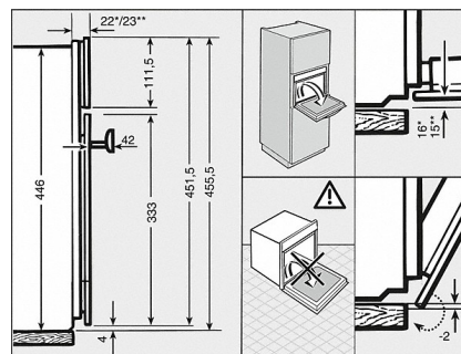
DG 6000 - detail drawing PureLine (Installation drawing)
