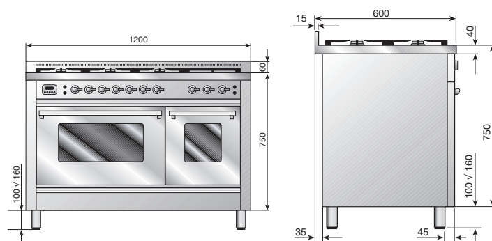
120cm Quadra 7 Burner Model PSW120FIE3 Total Electrical Load: 9.4kW Total Gas 'NG' Consumption 52.5 MJ/h
