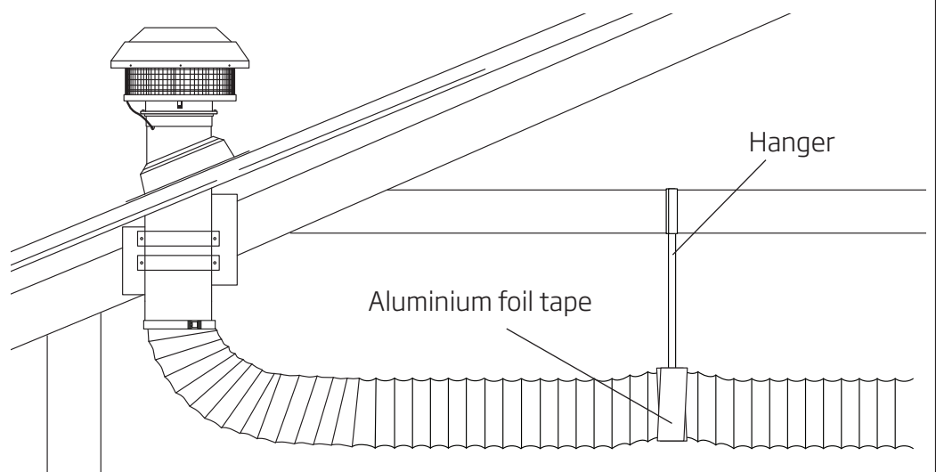
Figure 9: Securing SteelFlex™ Safety Duct
