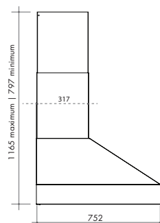
Technical Diagram Model: XBBQ90
