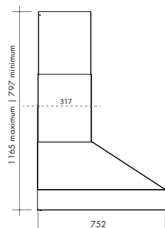
Technical Diagram Model: XBBQ120
