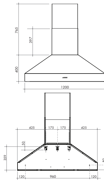
Technical Diagram Model: XBBQ120
