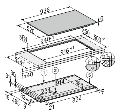
KM 7999 FL (installation drawing) - flush-fit
