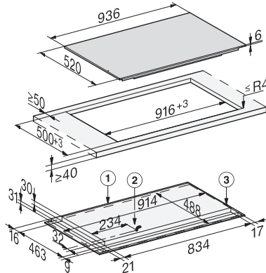
KM 7999 FL (installation drawing) - onset
