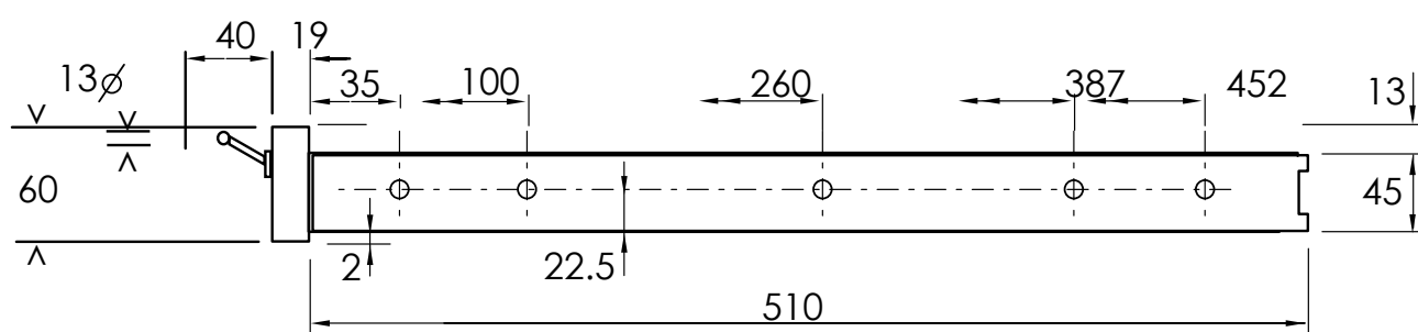
SIDE ELEVATION
