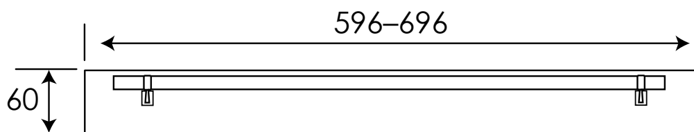
FRONT ELEVATION
