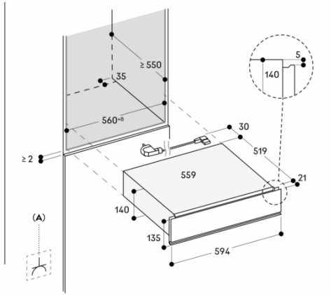
A: Accessible electrical connection Measurements in mm
