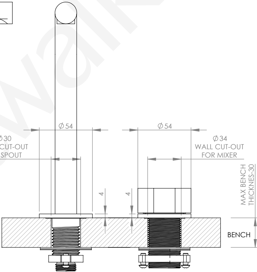
G 1/2" MALE SPOUT BASE
