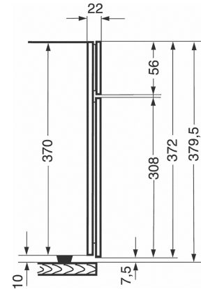
DG 1050, DG 1450, DG 6010, DG 6019clst (installation drawing)
