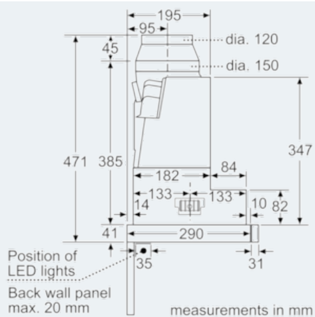
Dimensioned drawings
