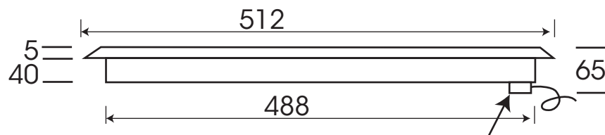
SIDE ELEVATION
