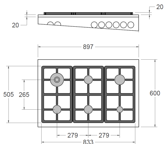
WORKTOP DETAILS
