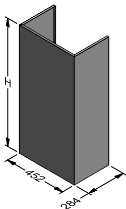
SMF 600L-1 SHROUD
