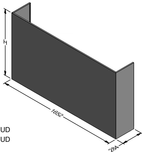
SMF 1800L-3 SHROUD
