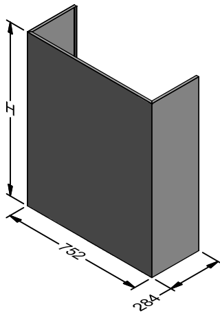
SMF 900L-1 SHROUD SMF 900L-2 SHROUD
