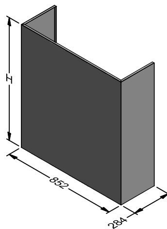
SMF 1000L-2 SHROUD
