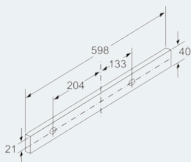
Dimensioned drawings
