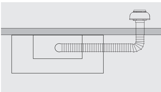
Top view for wall mounted installations on the same wall as the rangehood.
