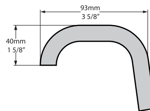
Rim detail
