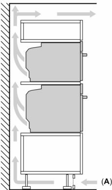
Installing two appliances on top of each other Air exchange
