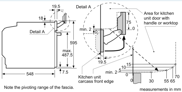
Measurements in mm Worktop thickness when installing underneath a hob (incl. substructure, if required)
