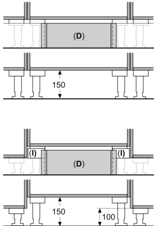
Measurements in mm Plinth variants for robot module
