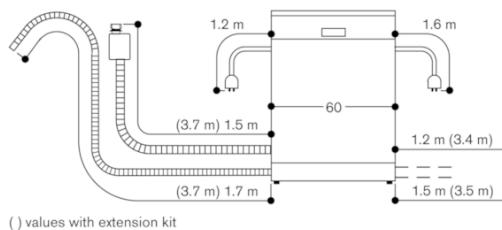
Connection dimensions for a 60 cm wide dishwasher
