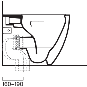
cod. 90 5455 0000 Adjustable pipe elbow fitting.
