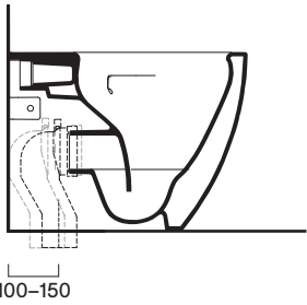
cod. 90 5456 0000 Adjustable pipe elbow fitting.
