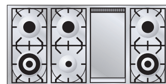
120cm Quadra 7 Burner Model PW120FMP Total Electrical Load (Kw) 5.7 Total Gas 'NG' Consumption (Mj/h) 76.3
