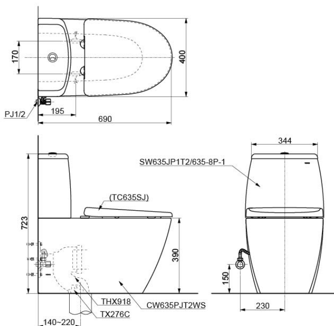
CW635PJT2WS / SW635JP1T2/635-8P-1
