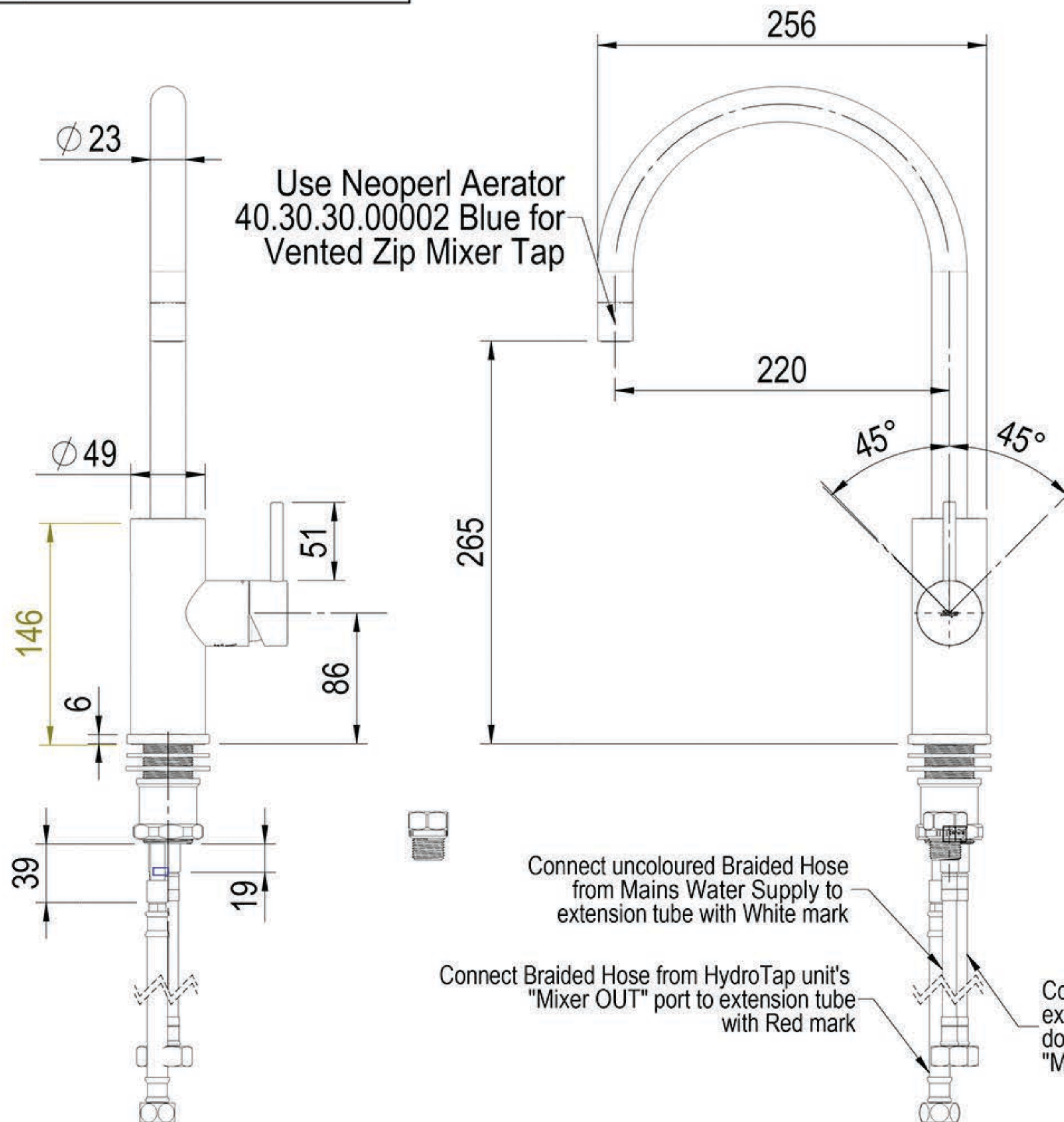
FRONT VIEW
