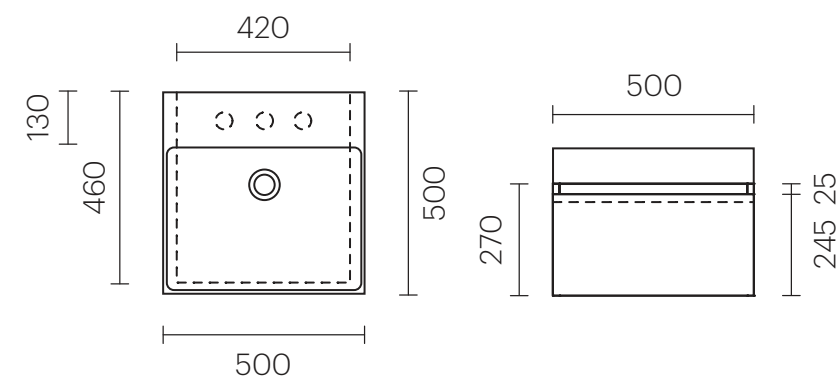
Top view with basin
