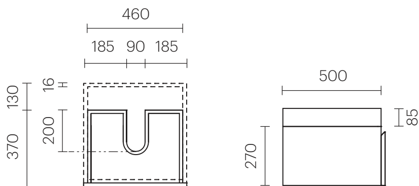
Top view cabinet only
