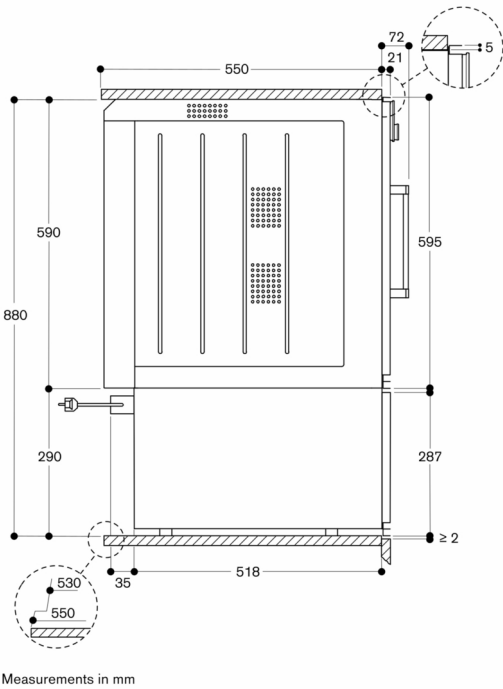
WSP 222 below BOP
