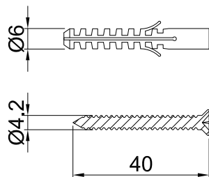
316 SCREW x 2
